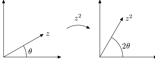
Figura 1.19: z \mapsto z^2 .
